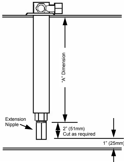
Low Profile Design HOT FOX™ fits where other fuel warmers can't.
